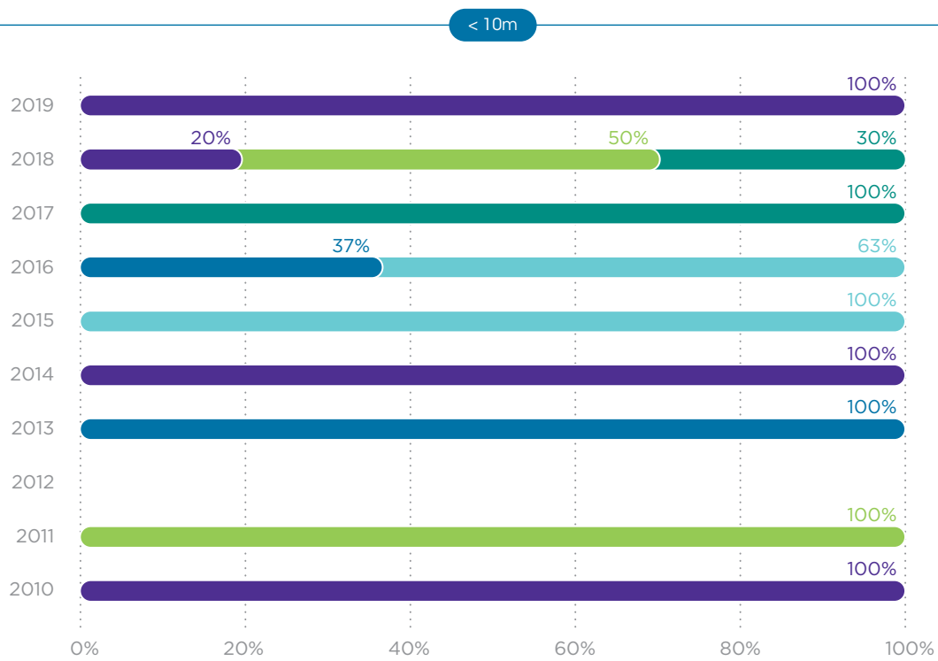
Figure 11. Share of installed capacity and water depth by foundation type (2010-2019)
