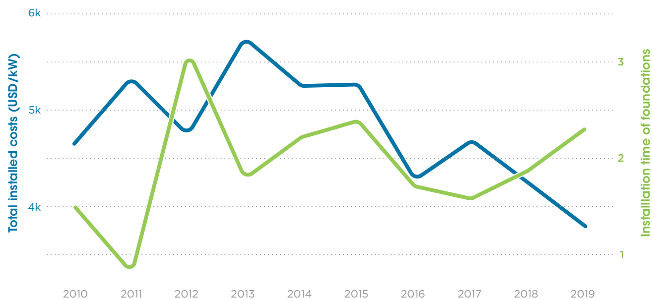
Figure 12. Installation time of foundations and total installed costs (2010-2019)
