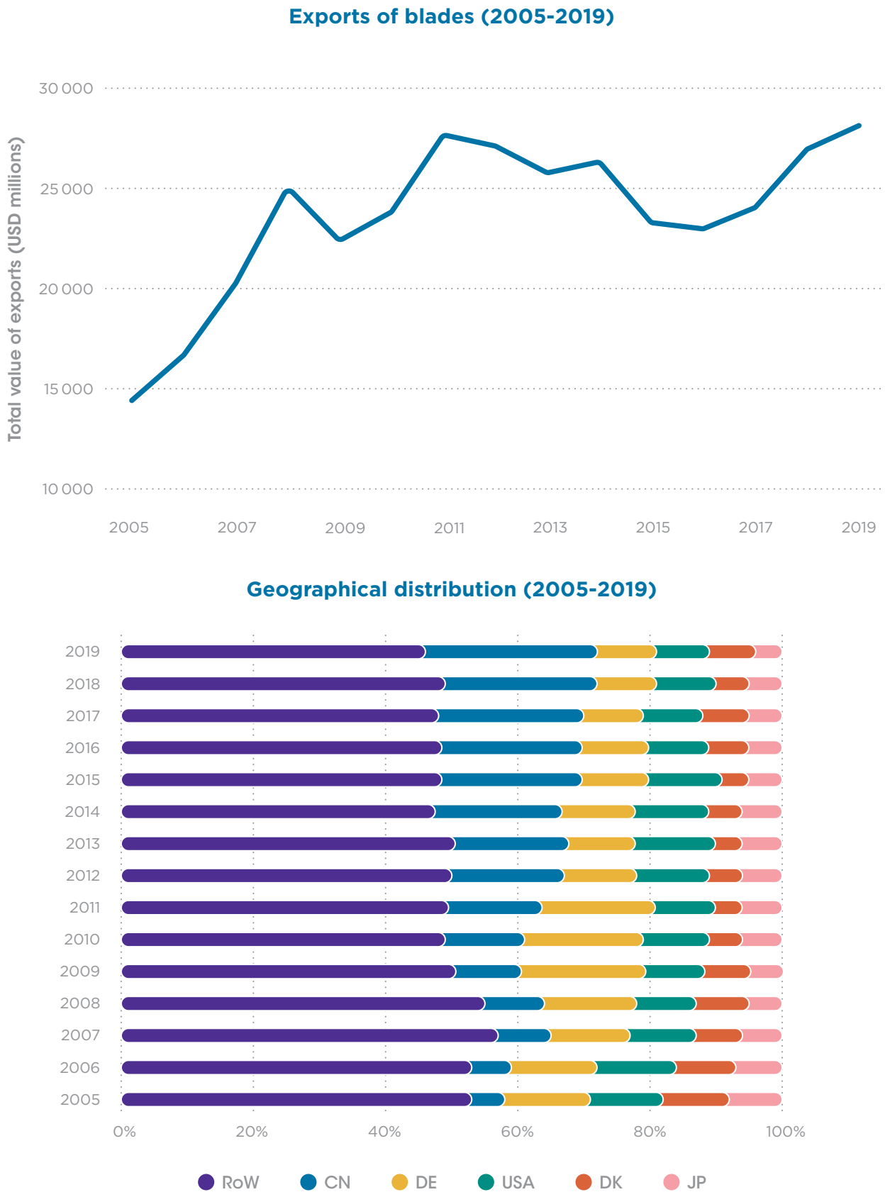
Figure 16. Blades exports and geographical distribution (2005-2019)
